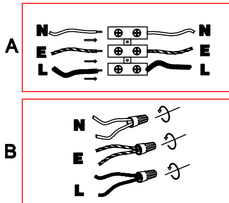
Wiring diagram
