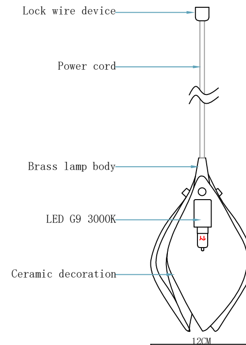
Single head schematic diagram
