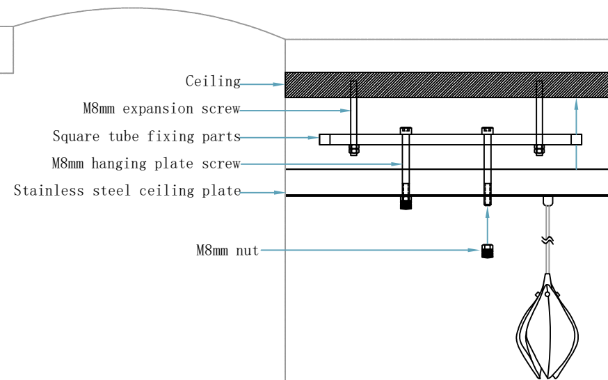
Enlarged Detail
