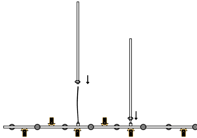
The round tube is locked to the lamp body
